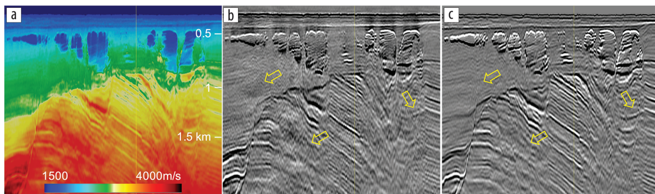
Figure 5. Section view of (a) the 40 Hz TLFWI model, (b) the 40 Hz Q -RTM, and (c) the 40 Hz FWI image from a source-over-spread NATS data set in the Barents Sea. Subgas reflectors and faults are better revealed in the FWI image in the areas indicated by the arrows.
