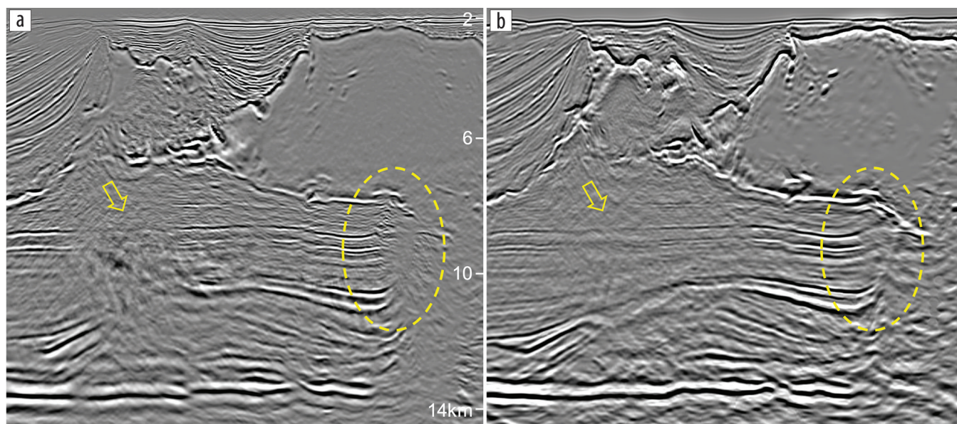
Figure 4. Section view of (a) the 15 Hz RTM image and (b) the 15 Hz FWI image from the corresponding 15 Hz TLFWI model for a WATS data set in Walker Ridge, GoM. The FWI image shows better event continuity in the areas right below complex salt (as indicated by the arrows) and at the steeply dipping three-way truncation (as highlighted by the ellipses).
