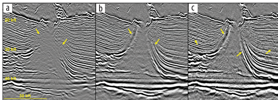
Figure 8. Comparisons of (a) 15 Hz RAZ RTM, (b) 15 Hz OBN RTM with dense nodes only, and (c) 15 Hz OBN RTM with dense and sparse nodes. The additional illumination from the long-offset OBN data provides better steep-dip imaging. The sparse nodes provide further illumination along the feeder flanks, but they also bring increased noise (seen within the basins, within the salt body, and at basement level).
