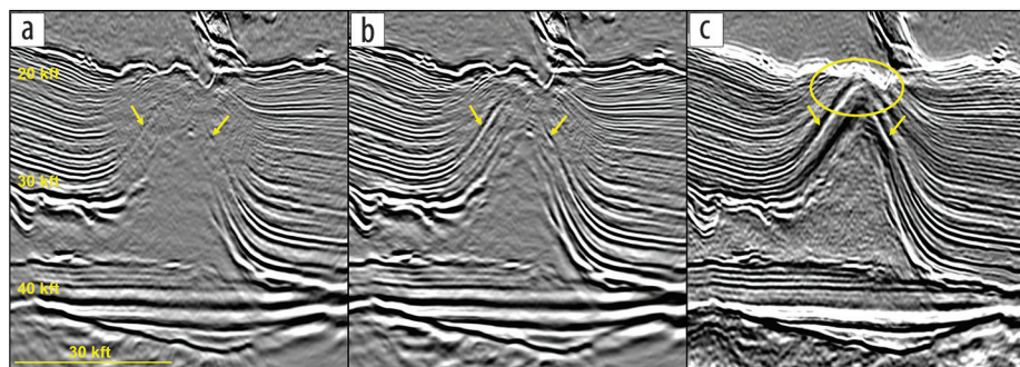
Figure 9. (a) 15 Hz OBN RTM. (b) 15 Hz OBN LSRTM. (c) 15 Hz FWI image. Illumination remains poor even with OBN data, but LSRTM provides some compensation for the weak amplitudes along the steep flanks of the feeder. The best compensation is provided by the FWI image. An estimate of the reflectivity comes directly from the FWI velocity model. The poorly illuminated events (steep dips and basement) show more balanced amplitude, and the steep dips extend all the way to BOS.
